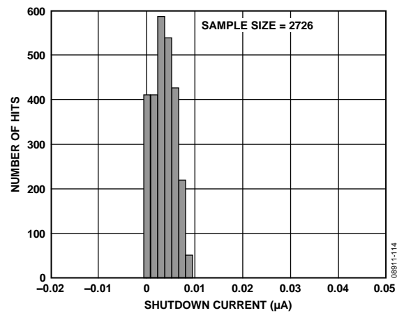
Figure 14. Supply Current, Power-Down Mode
